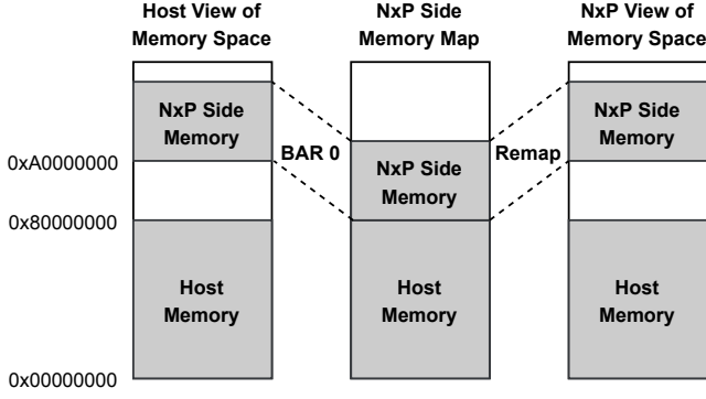
Fig. 3. The host system and NxP platform share the same physical address space through remapping of the BAR region on the NxP side.
