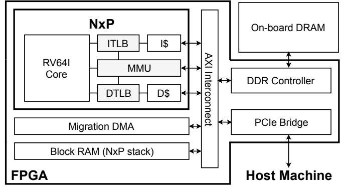
Fig. 4. FPGA-based evaluation platform for Flick.
