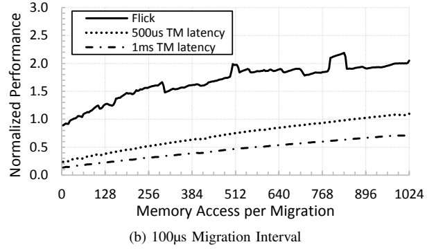
Fig. 5. Pointer chasing microbenchmark with different thread migration latency and migration interval.
